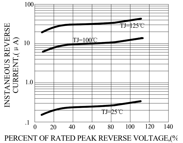
FIG.4-TYPICAL REVERSE CHARACTERISTICS
